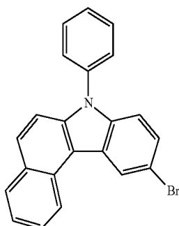
compound 2
