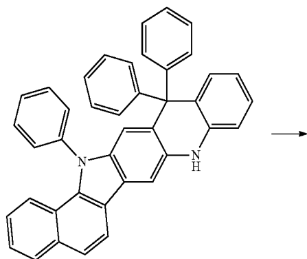
compound 4
