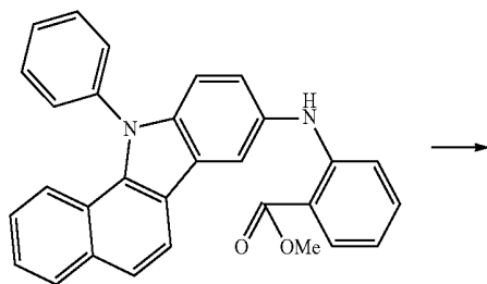
compound 2
