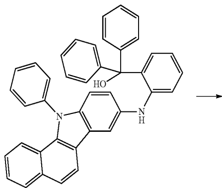
compound 3
