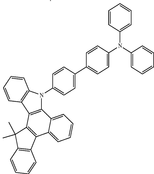
Formula 1-6-5
