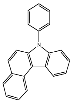
compound 1
