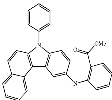
compound 3
