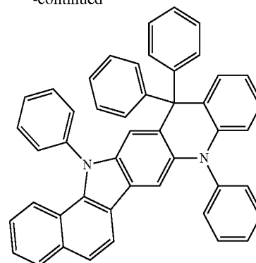
Formula 1-2-14
