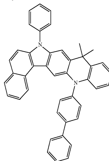
Formula 1-4-2
