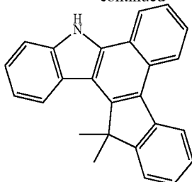
compound 3
